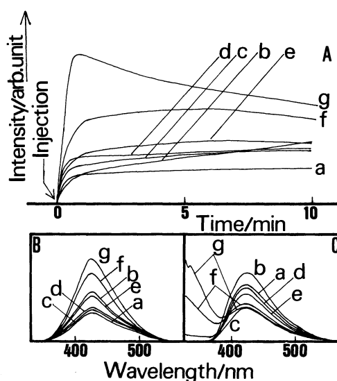
Fig. 6. Time course of luminol chemiluminescence (A), chemiluminescence spectra at 10–12.5 min after the initiation of the reaction (B) and fluorescence spectra of the total reaction mixture at 48 h after the initiation of the reaction (C) with and without surfactants. [Luminol] = 8.0 \times 10^{-5} \text{ mol dm}^{-3} in 0.1 \text{ mol dm}^{-3} \text{ Na}_2\text{CO}_3 . [ \text{H}_2\text{O}_2 ] = 0.10 \text{ mol dm}^{-3} . [ \text{K}_2\text{S}_2\text{O}_8 ] = 2.5 \times 10^{-4} \text{ mol dm}^{-3} . [Surfactant]/ \text{mol dm}^{-3} : a; surfactant free, b; [CTAB] = 1.8 \times 10^{-3} , c; [SDS] = 1.6 \times 10^{-2} , d; [Brij 35] = 2.0 \times 10^{-4} , e; [Triton X-100] = 8.0 \times 10^{-4} , f; [Triton X-100] = 8.0 \times 10^{-3} , g; [Triton X-100] = 2.0 \times 10^{-2} . a–e: cmc \times 2 , f: cmc \times 20 , g: cmc \times 50 . These cmc values are in water (Refs. 6, 8).
